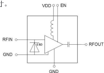
Block Diagram
